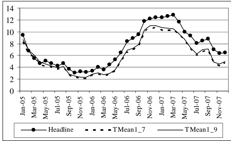
Figure 2: Trimmed Mean Measures and Headline Inflation
