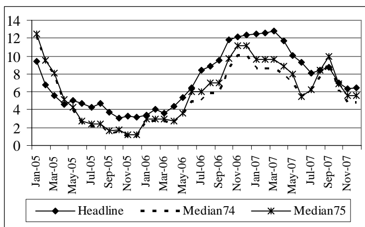
Figure 4: Weighted Medians and Headline Inflation
