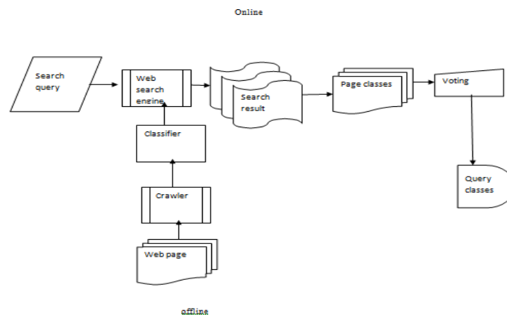
FIGURE 7. Architecture Of Search Engine
