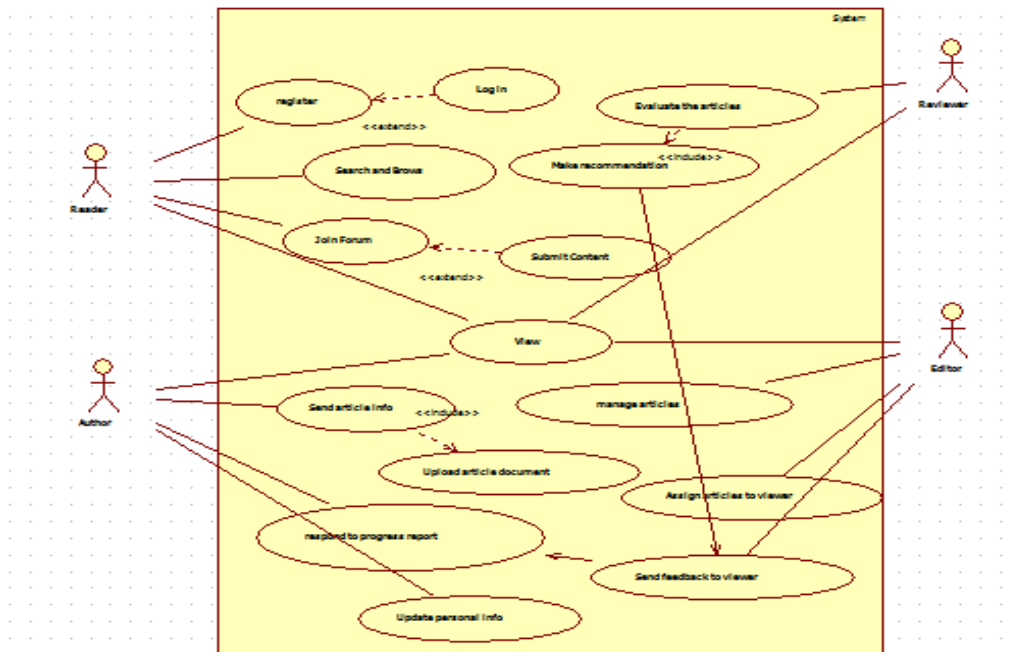
FIGURE . Use Case Diagram
