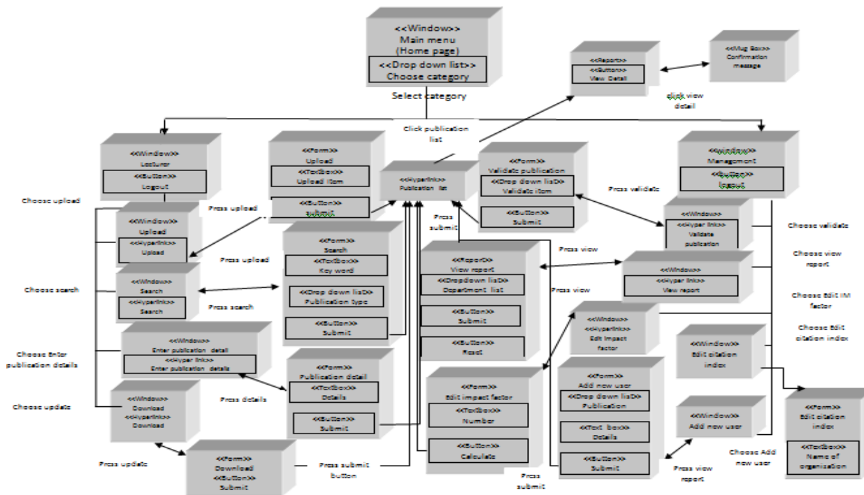
FIGURE 6. WINDOWS NAVIGATION DIAGRAM
