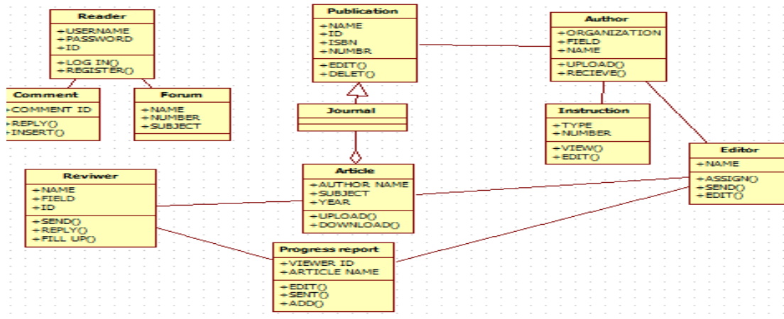
Figure 5:Class Diagram
