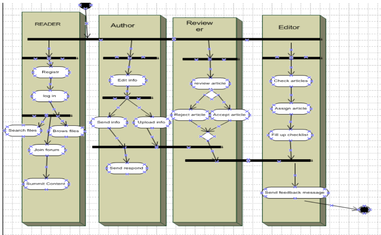
FIGURE 4. Activity Diagram
