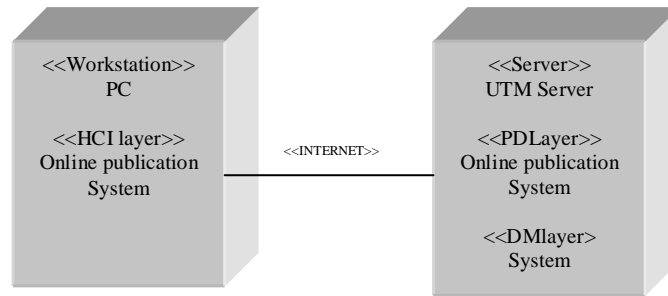
Figure 2 . Architecture of system
